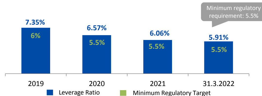
Leverage Ratio
